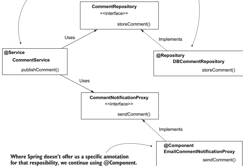
Figure 4.12 We use the @Service and @Repository annotations to explicitly mark the responsibilities of the components in our class design. Where Spring doesn't offer a specific annotation for that responsibility, we continue to use @Component .
